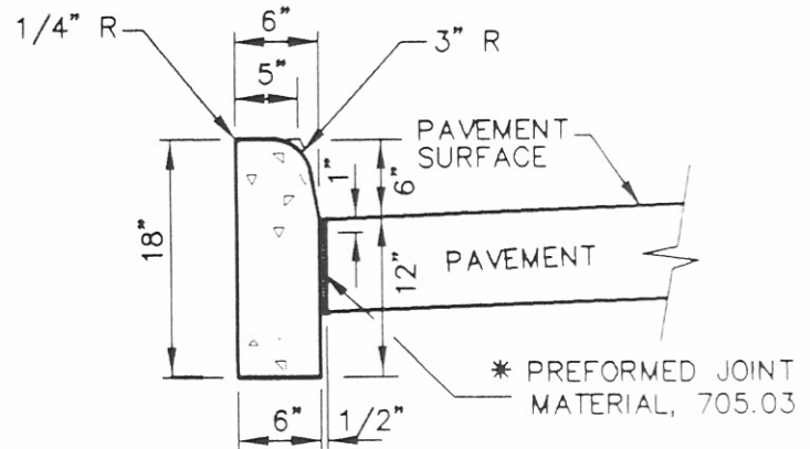
TYPE 6-CONCRETE CURB
