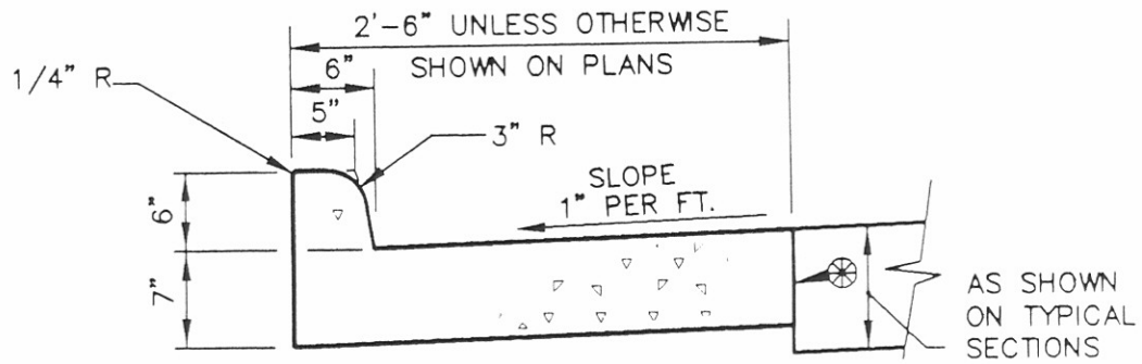
TYPE 2 COMBINATION CONCRETE CURB & GUTTER
