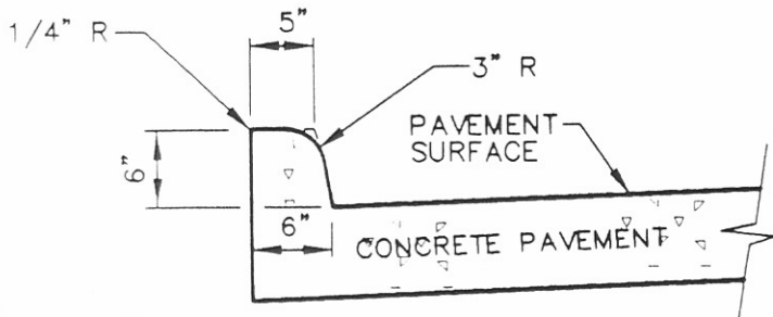
TYPE 2A-INTEGRAL CONCRETE CURB
