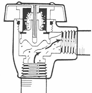
ATMOSPHERIC VACUUM BREAKER No. 288A
